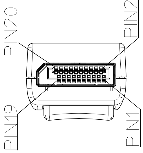
PINOUT DETAIL
